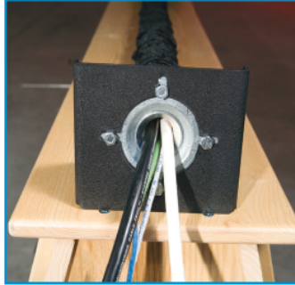
2. Feed Wires
