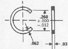
RETAINING RING For use with all size 4 studs
