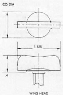
STUD, WING HEAD DP 137-1W
