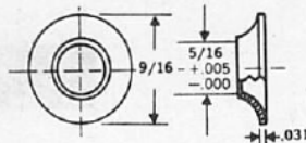
TYPE GH HALF GROMMET Installed View, P. 28
