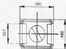
STUD HEAD SLOT ALIGNMENT IN LOCKED POSITION
