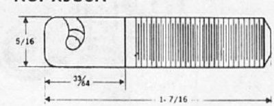
NO. X936A 5/16"-18 Thread, UNC-2A
