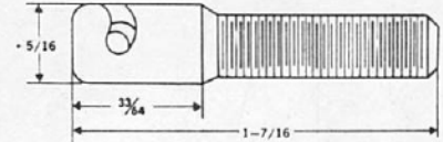
NO. X936A 5/16"-18 Thread, UNC-2A
