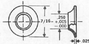
GH HALF GROMMET For use with all size 4 studs
