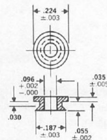
SPACER For use with URFA4 Floating Receptacle 2 supplied with each receptacle
