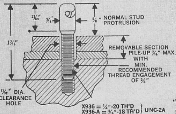
FIG. 1 - BLIND HOLE MOUNTING USING THREAD LOCKING COMPOUND
