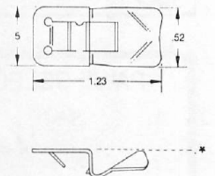
PAWL DP 137-2S DP 137-2L
