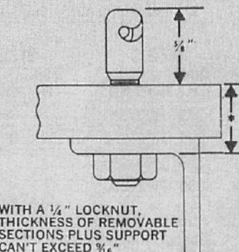
FIG. 2 - BLIND HOLE APPLICATION USING JAM NUT
