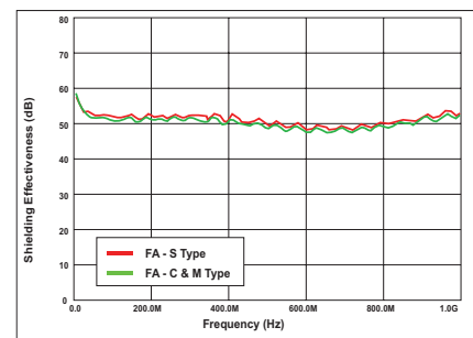
Typical SE in S, C, & M Type Construction
