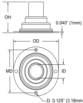
"B" Bellow Seal
