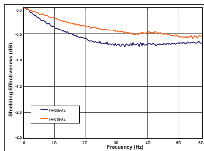
Typical Absorption in A Type Construction
