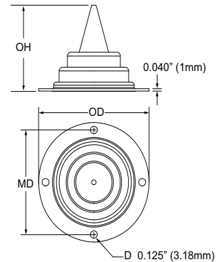
"D" Pointed Bellow Seal
